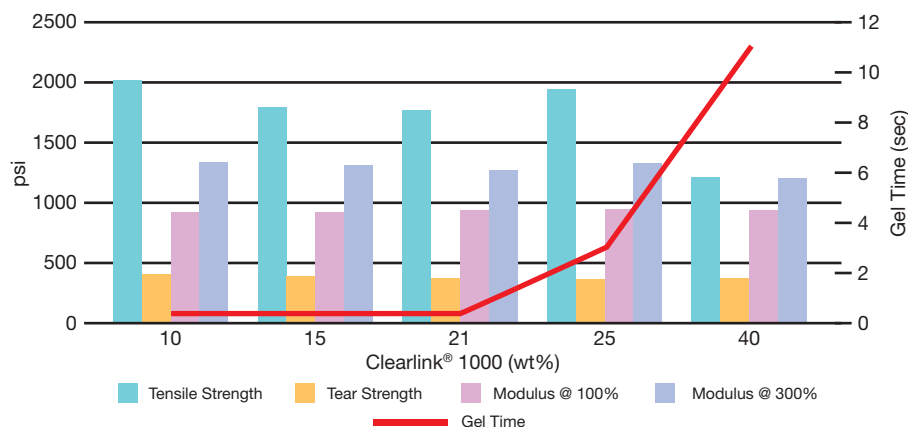
Tensile Strength, Tear Strength, Modulus and Gel Time Sprayed Polyurea Coating with Clearlink® 1000
